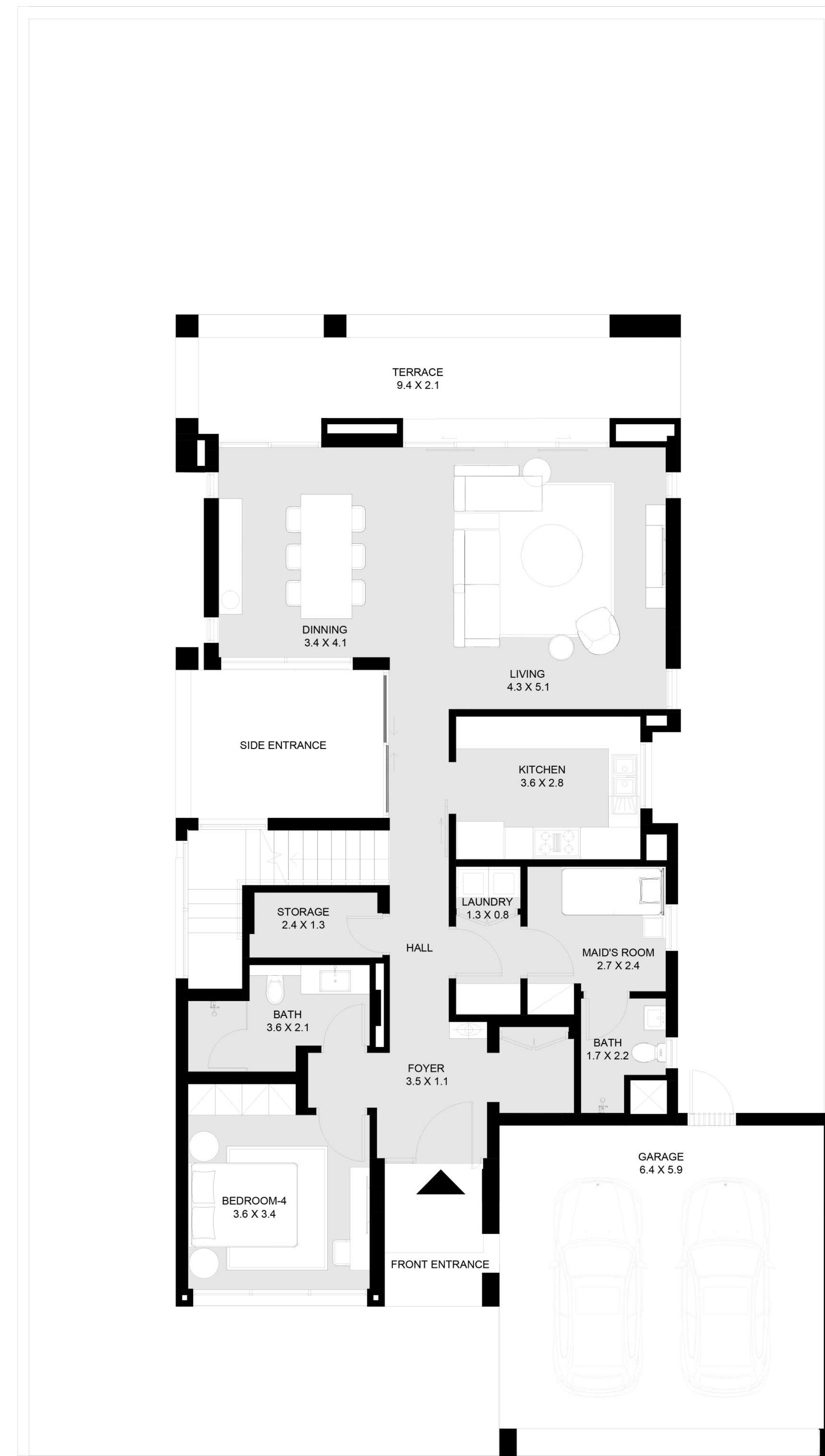
GROUND FLOOR
