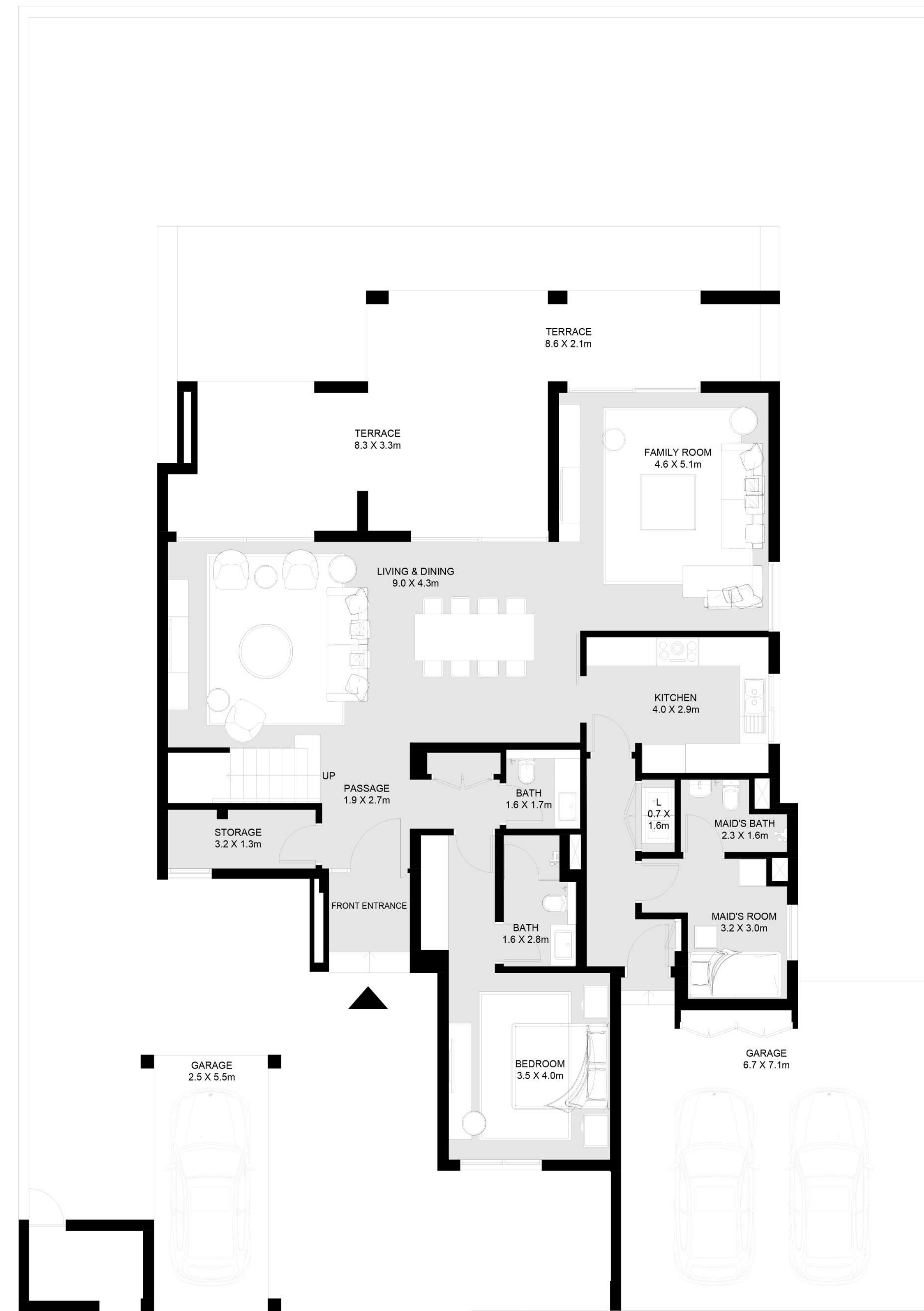
GROUND FLOOR
