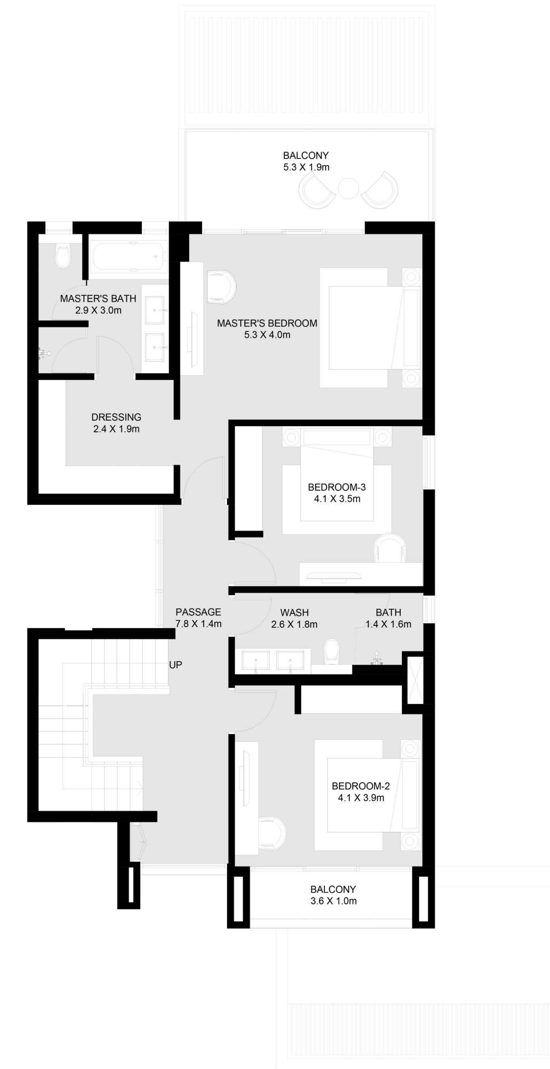
FIRST FLOOR
