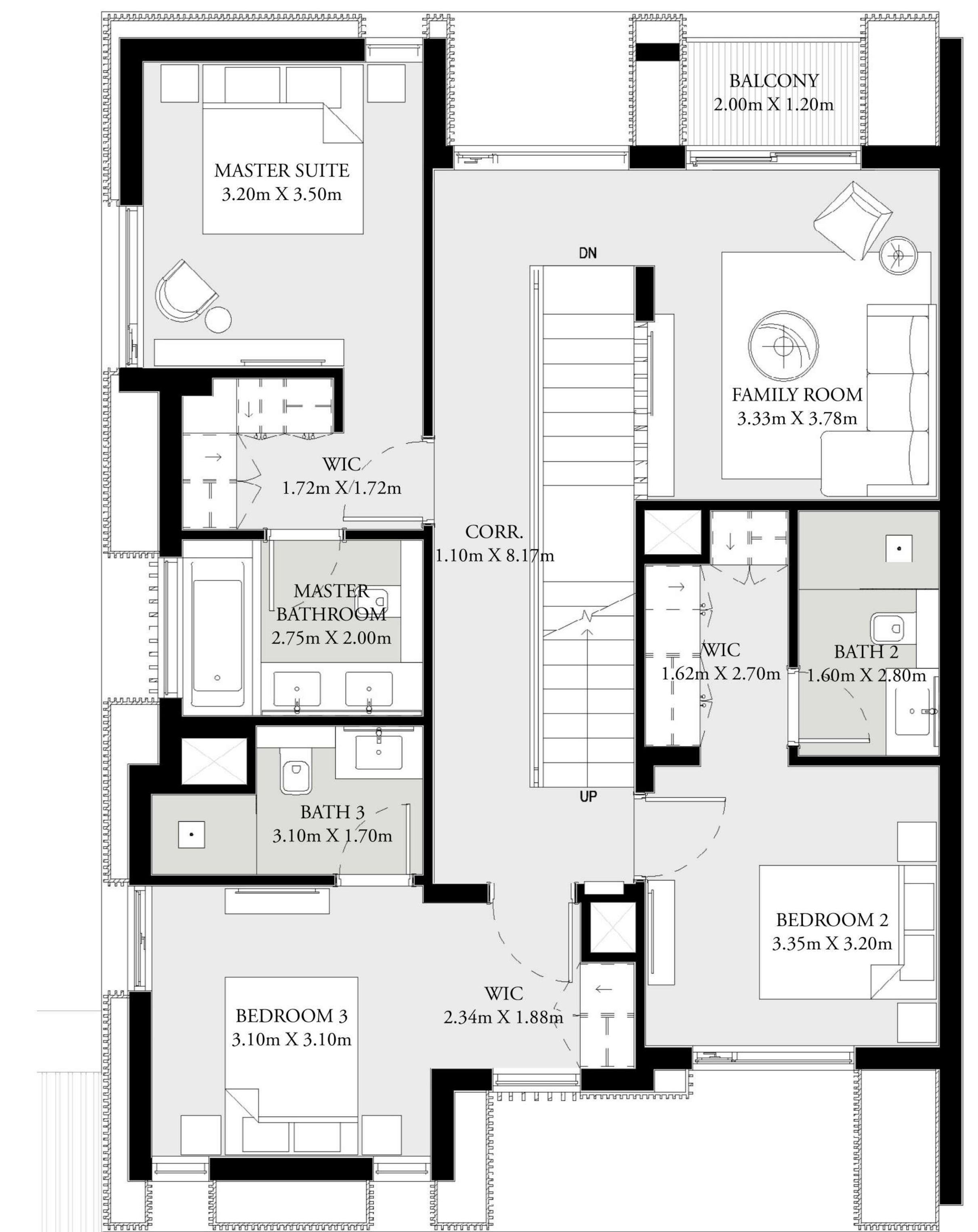
FIRST FLOOR
