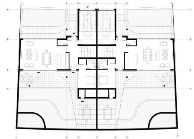
LEVEL 1
